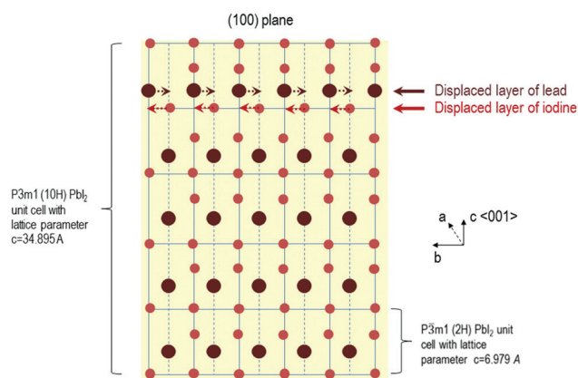
Fig. 4 Schematic illustration of the change in space group from P3m1 (shown for the 10H polytype) to P3m1 for \text{PbI}_2 nanosheets with the growth time.
